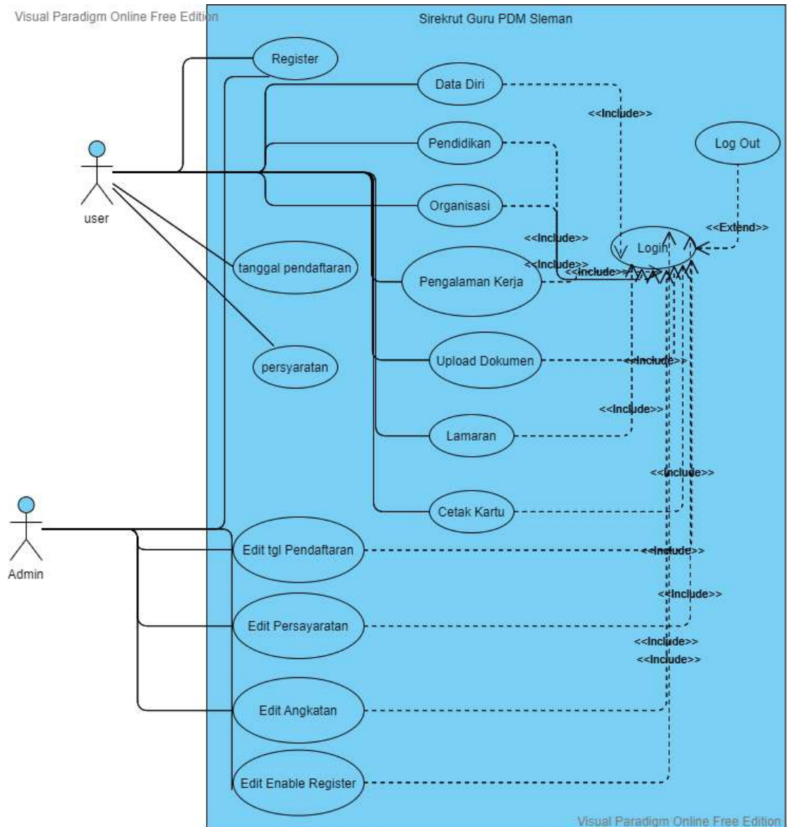
Gambar 1 Use Case Diagram
